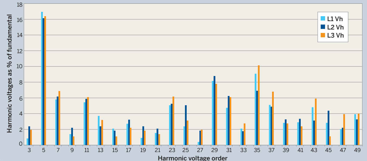
Offshore platform harmonic voltage spectrum
